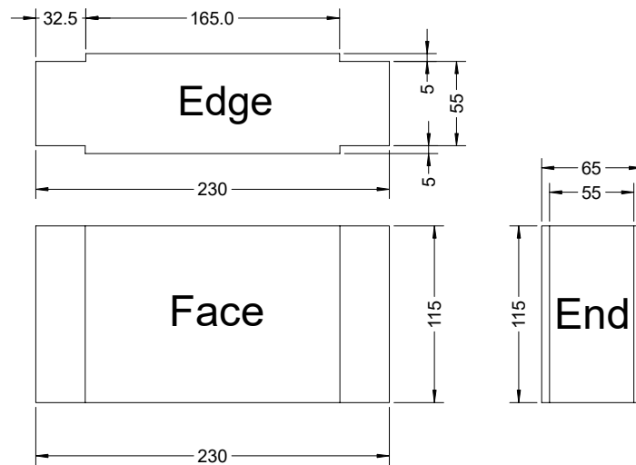
Bricks, 4 cut-outs
