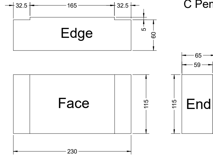
Bricks, 2 cut-outs
